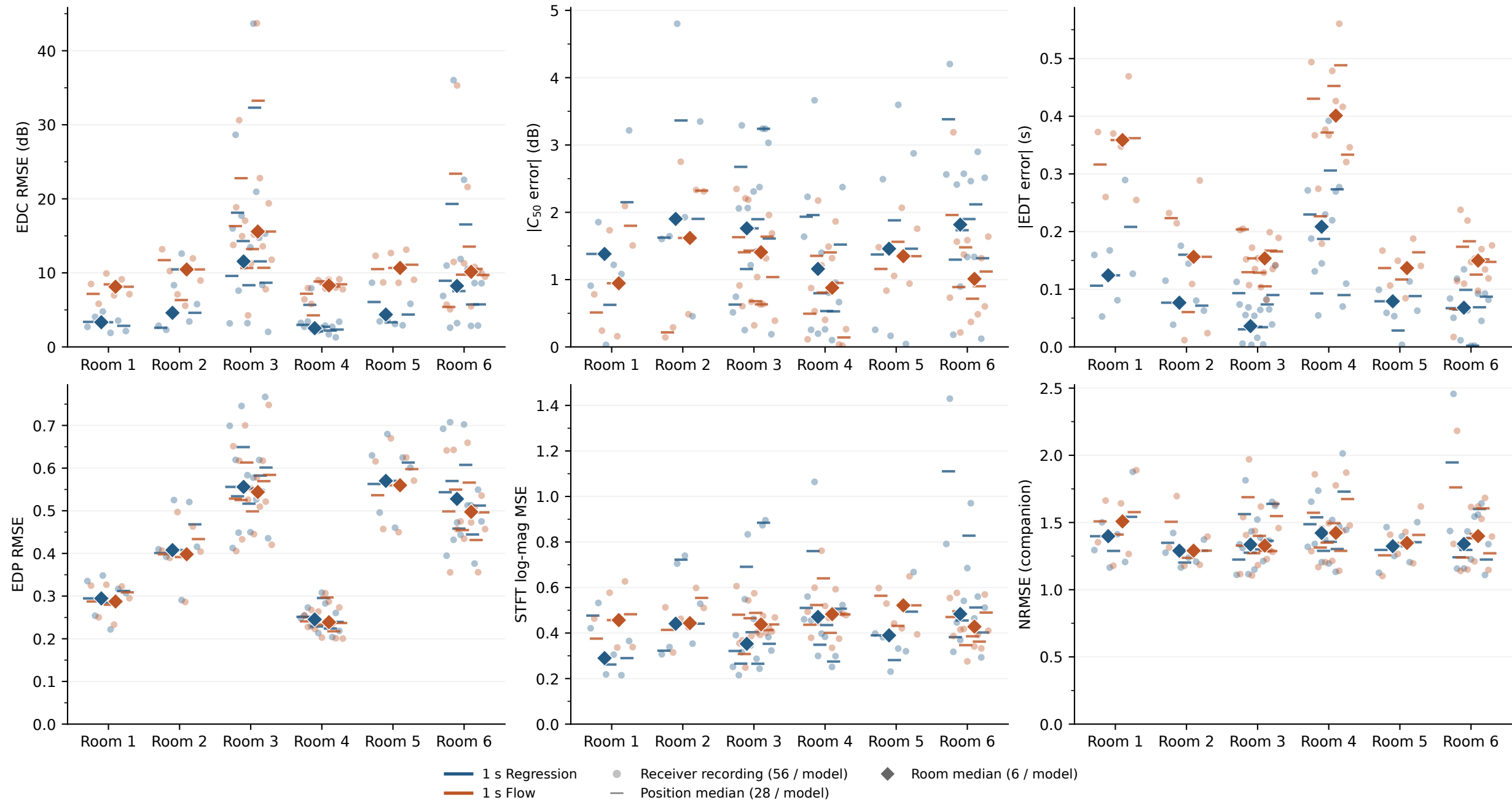
ARPEGE: paired external transfer against measured RIR references
