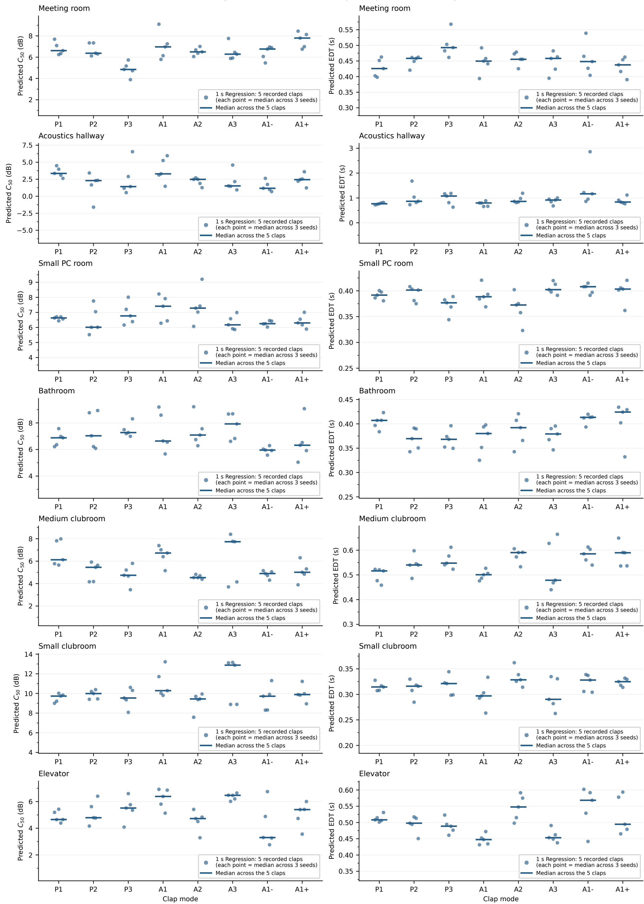
E6: 1 s Regression; no reference RIR — panel-specific vertical ranges
