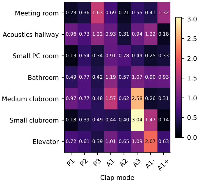
Within-room C50 deviation (dB)
