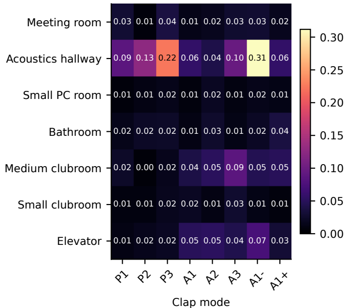
Within-room EDT deviation (s)
