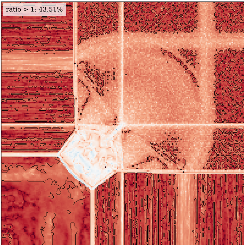
HLLC p16 rho
