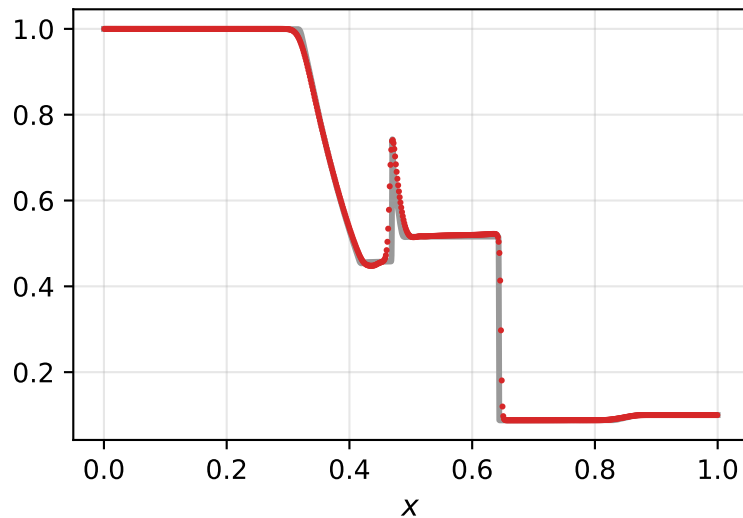
Pressure p
