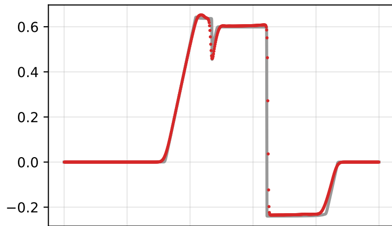
Velocity v_x
