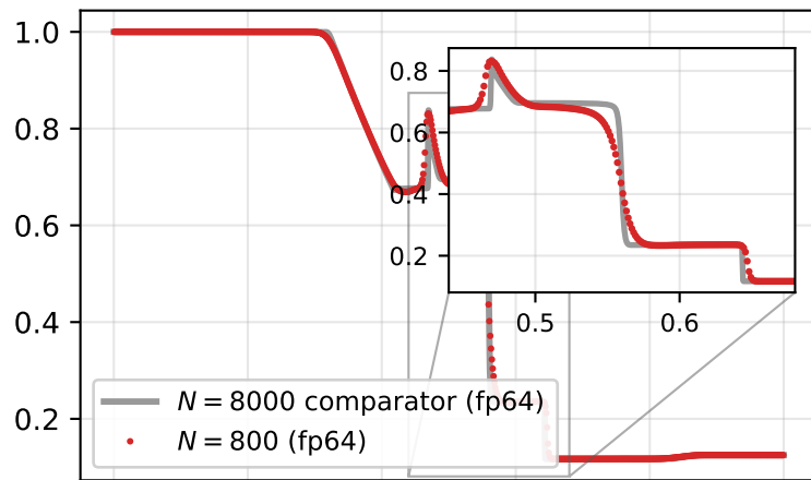
Density \rho
