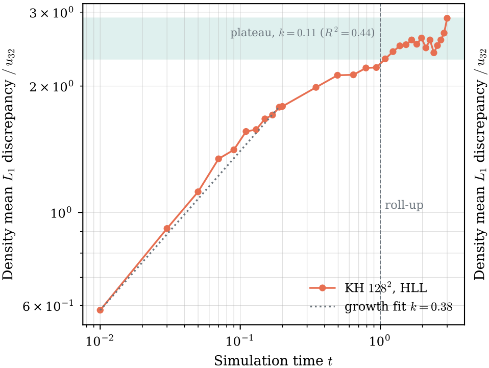
(a) Kelvin-Helmholtz through roll-up
