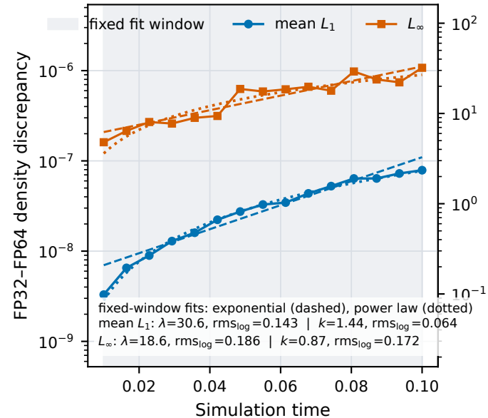
(a) Brio-Wu
