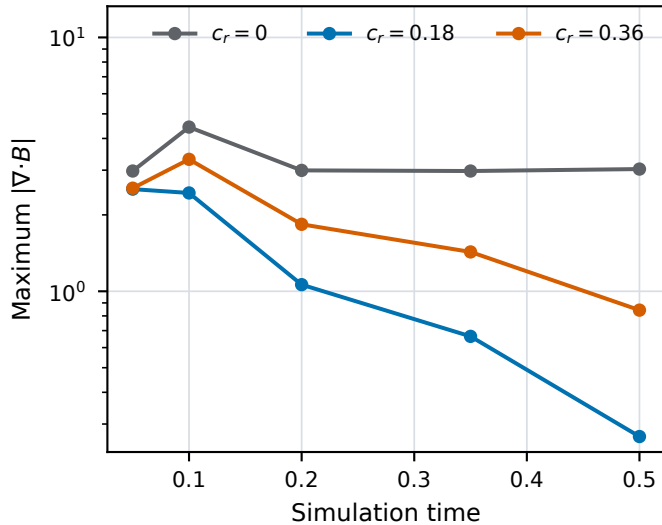
GLM cleaning, 128^2 Gaussian B_x bump
