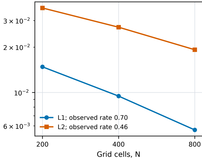
Brio-Wu numerical-reference refinement
