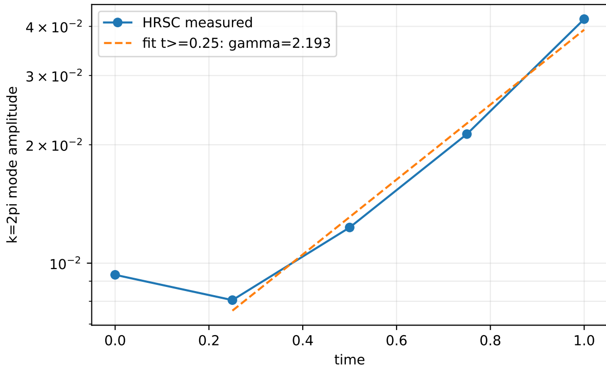
Lecoanet KH early linear-growth reproduction
