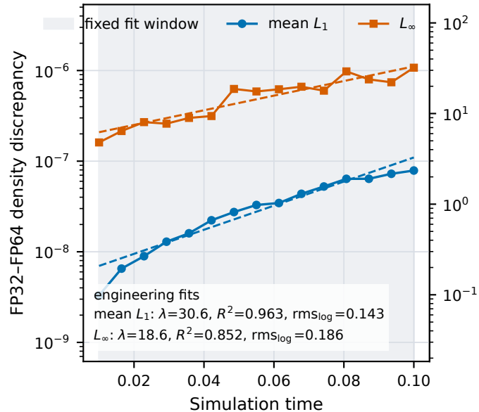
(a) Brio-Wu
