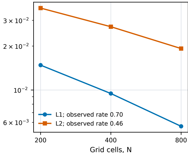
(a) Brio-Wu numerical-reference refinement
