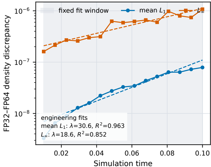
(a) Brio-Wu
