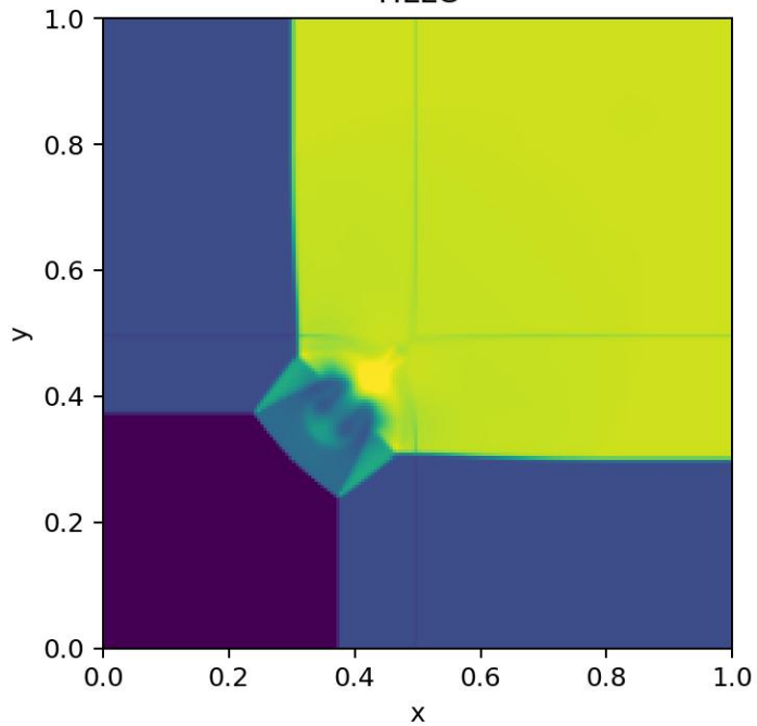
HLLC
