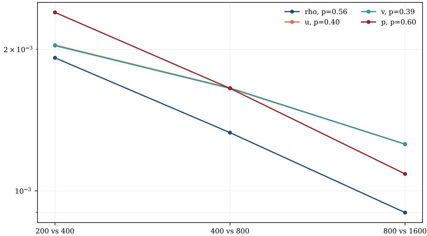
LW12 fp64 self-convergence against finer grids
