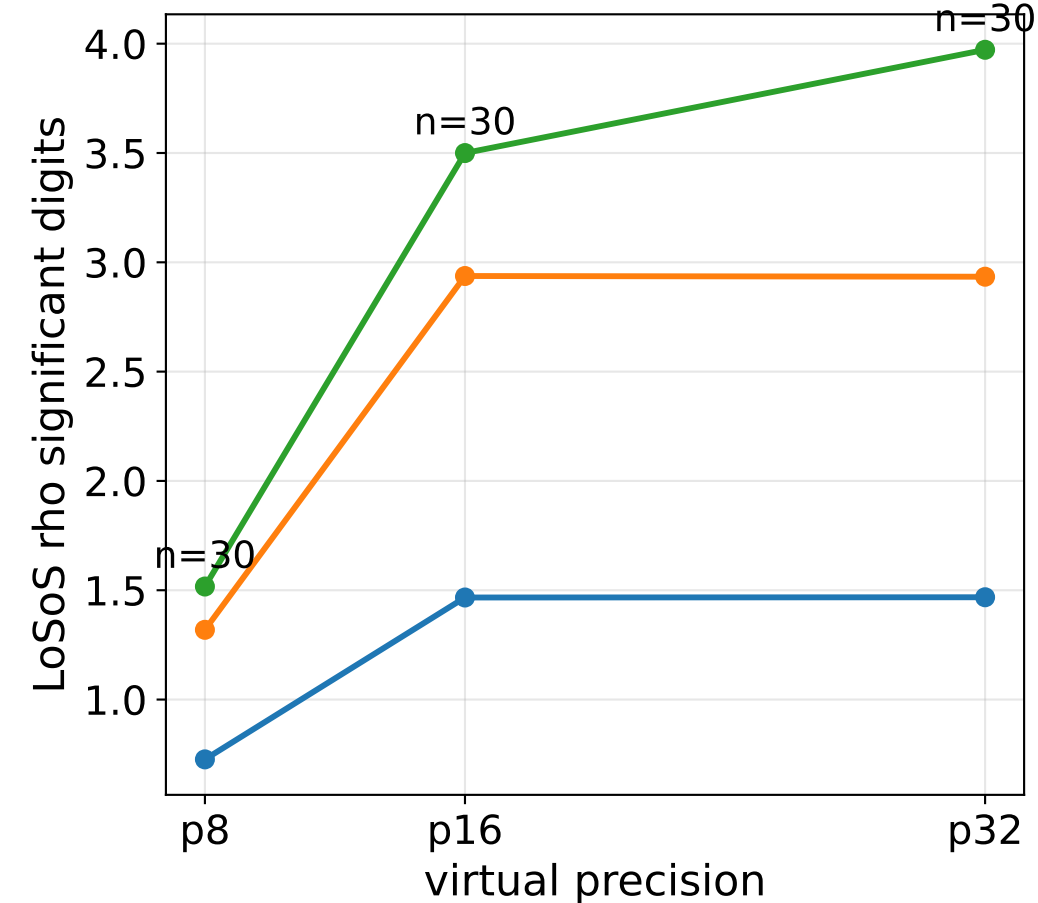
HLLC
