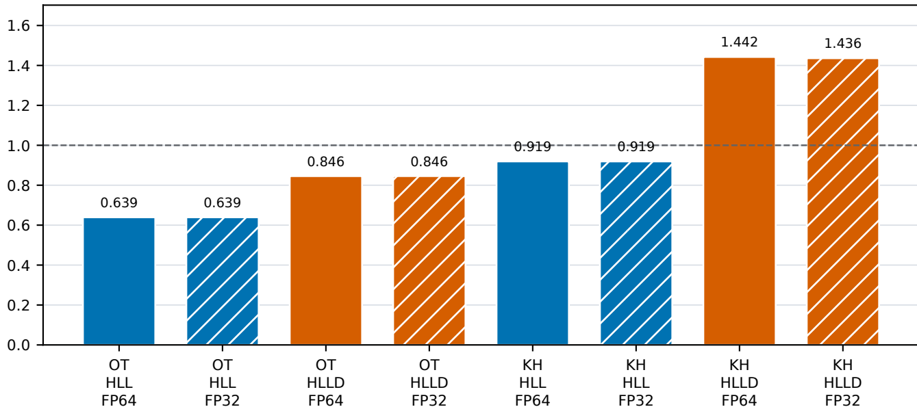
Three-grid MHD self-refinement diagnostic
