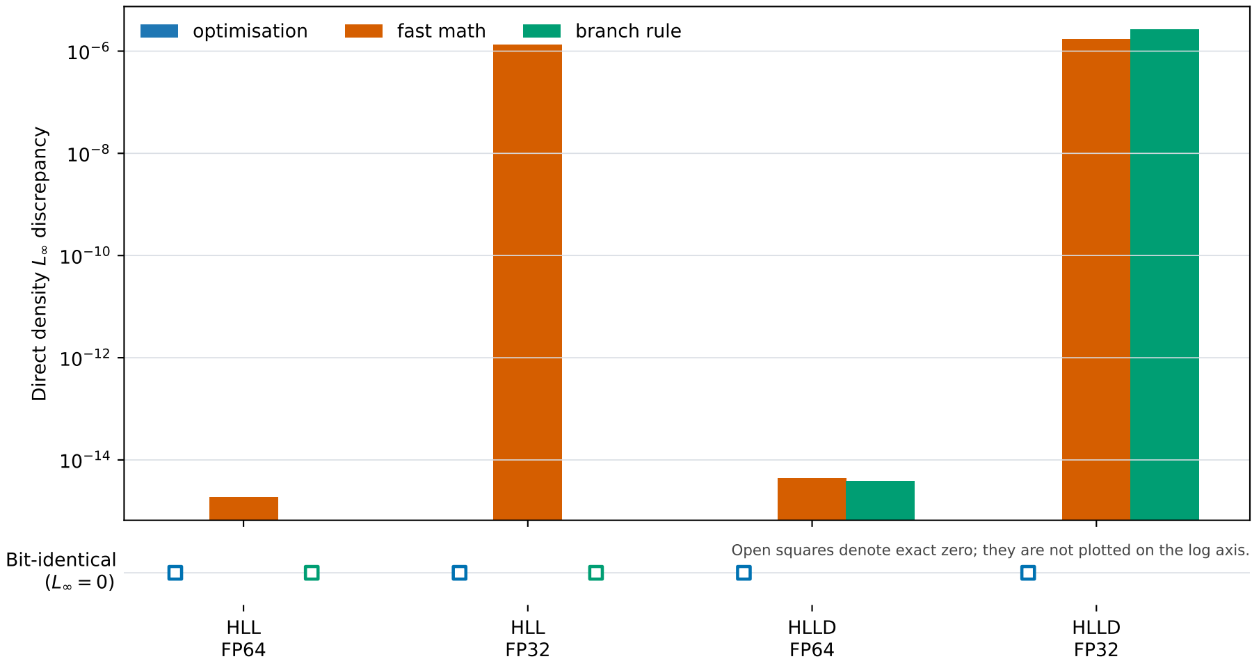
Brio--Wu: positive build-semantics responses (log scale)
