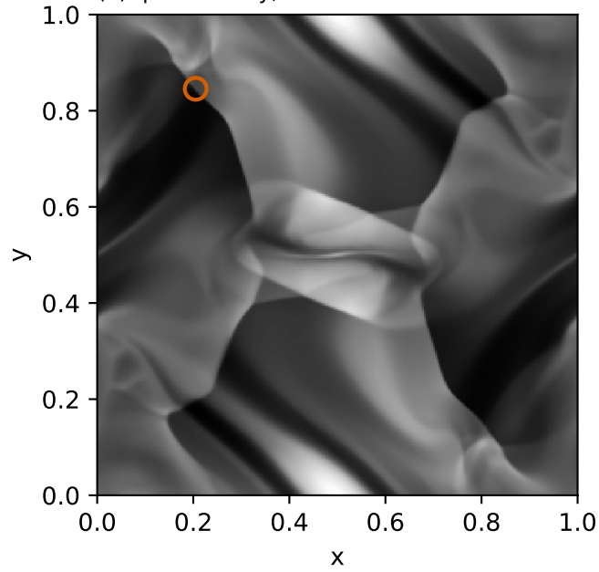
(a) fp64 density, HLLD 256^2
