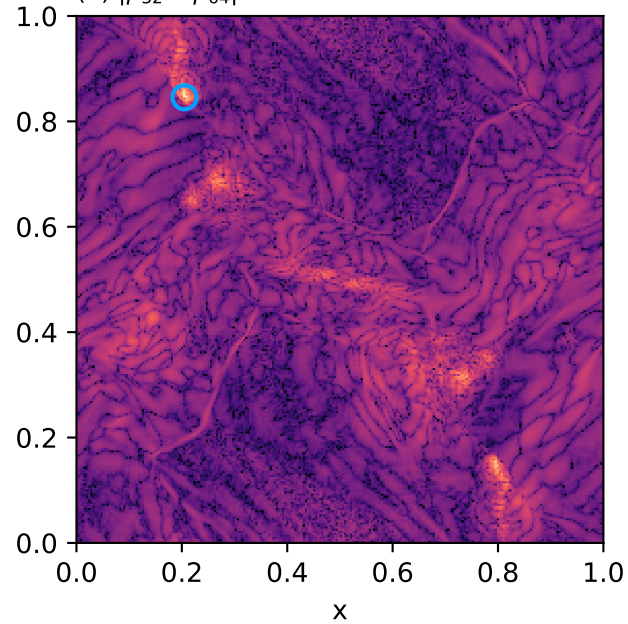
(b) |\rho_{32} - \rho_{64}|
