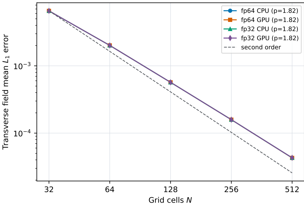
Circularly polarised Alfvén wave at t = 1
