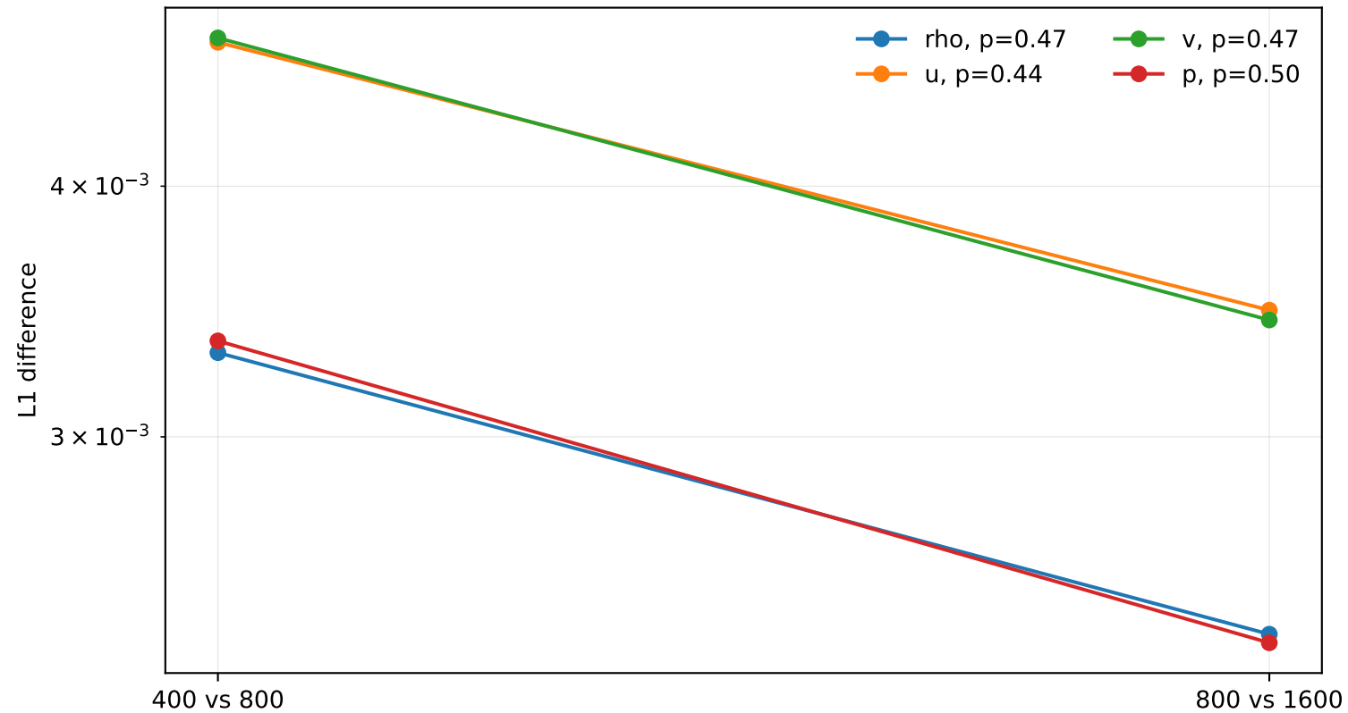
LW3 fp64 self-convergence against finer grids
