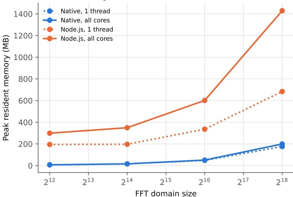
Peak memory vs circuit size
