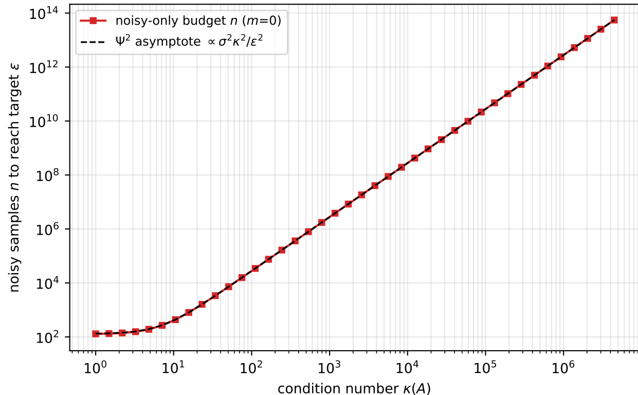
noisy-only budget diverges with \kappa ( \Psi -driven)
