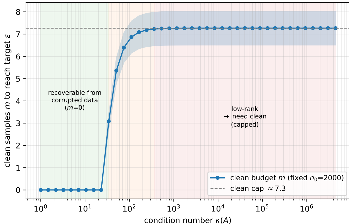
D2: clean budget vs condition number
