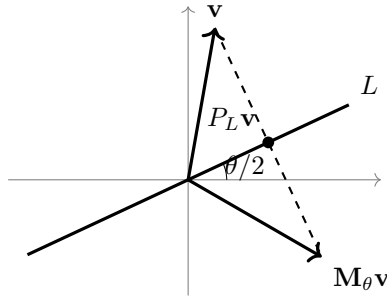
\mathbf{M}_\theta reflects in the line L at angle \theta/2
