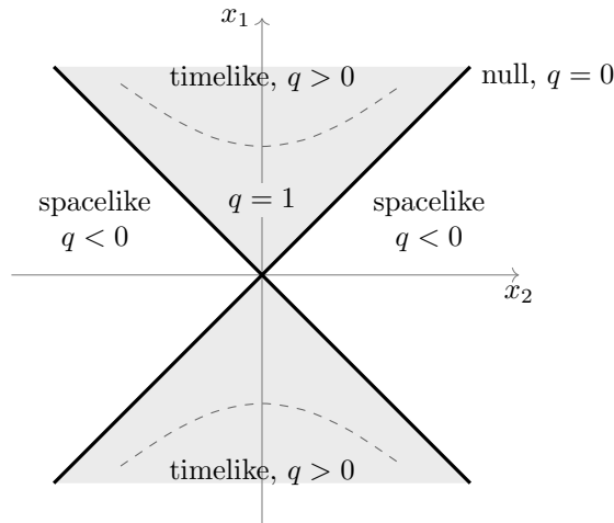
The light cone q = 0 in the Minkowski plane separates the timelike vectors from the spacelike ones; the “unit sphere” q = 1 is the dashed hyperbola, and it is unbounded
