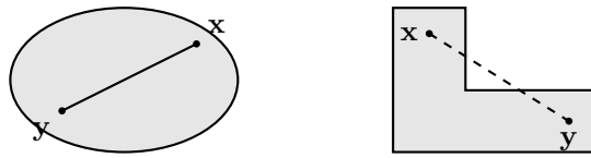
convex not convex: the dashed segment leaves the set
