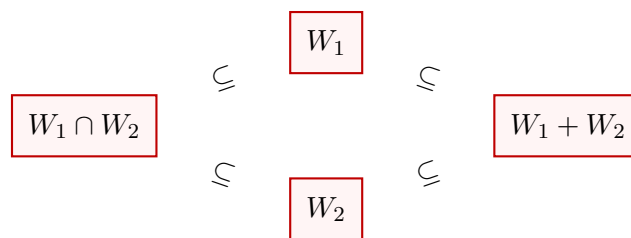
Inclusion diagram for subspaces W_1 and W_2
