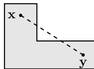
convex not convex: the dashed segment leaves the set
