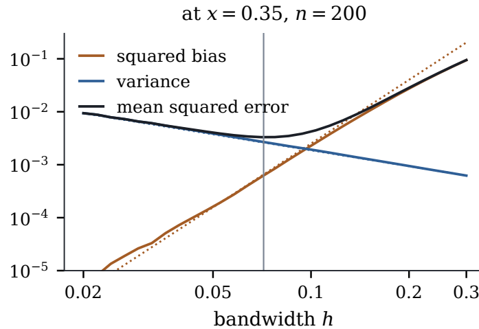
Figure 43.1.2: Squared bias, variance and mean squared error of the local linear estimate at x = 0.35 against the bandwidth, from 2000 data sets (solid) and from Theorem 43.1.3(a) (dotted); the vertical line is h^* . Logarithmic scales.
