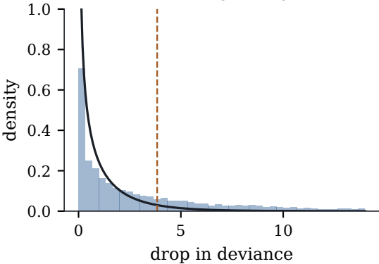
(a) naive, against \chi^2(1)
