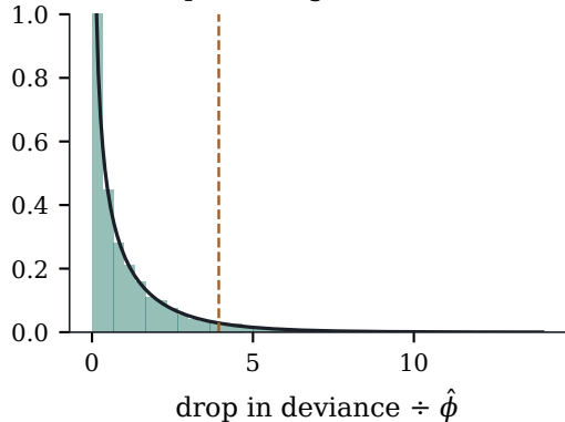
(b) quasi- F , against F(1, 98)
