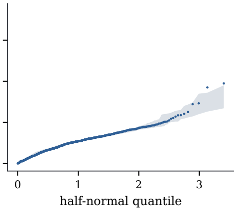
(b) beta-binomial
