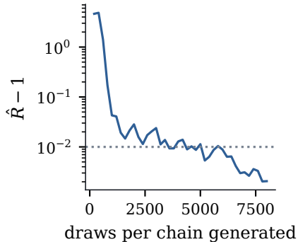
(b) convergence
