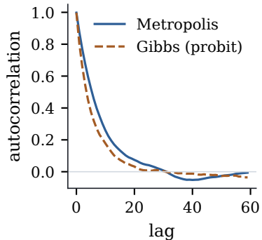
(c) mixing
