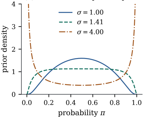
(a) what a normal prior implies
