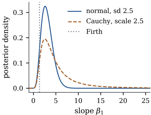
(b) the separated subgroup
