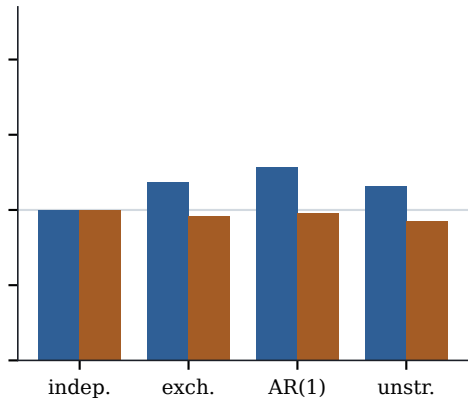
(b) AR(1) truth, \rho = 0.8
