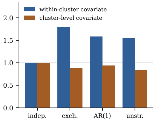
(a) exchangeable truth
