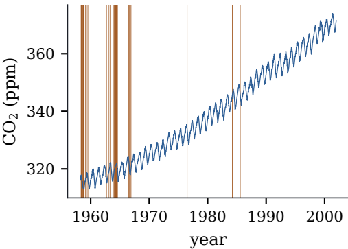
(a) weekly record, gaps marked
