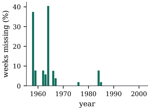
(b) missing fraction by year
