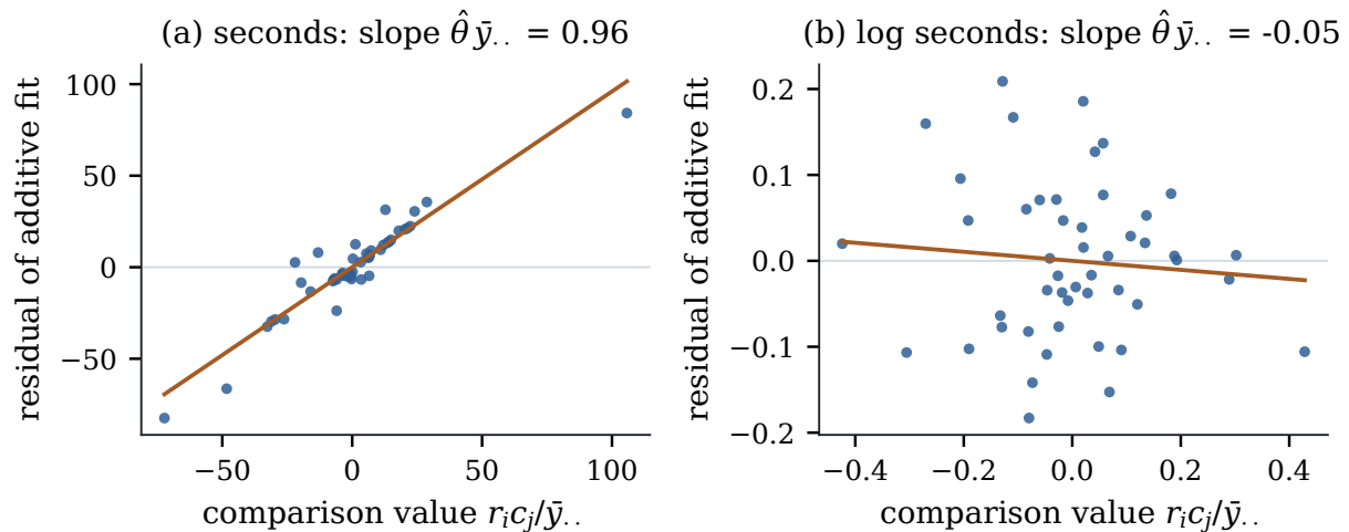
Figure 16.1.1: Tukey's diagnostic plot for the solver data: residuals of the additive fit against the comparison values r_{ij}\bar{c}_j/\bar{y}_{..} , with the fitted line of slope \hat{\theta}\bar{y}_{..} = 1 - \hat{p} . (a) In seconds the residuals lie along a line of slope near one, which points to the logarithm. (b) In log seconds there is no trend.
