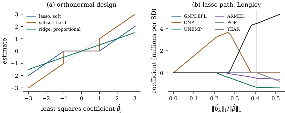
Figure 27.4.1: (a) Lasso (soft thresholding), subset selection (hard thresholding) and ridge regression (proportional shrinkage) as functions of the least squares coefficient under an orthonormal design, with \lambda = 1 (Theorem 27.4.2). (b) The lasso path for the standardized Longley data; the vertical line marks the leave-one-out choice of \lambda .
