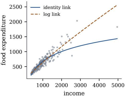
(a) two links, same regressors
