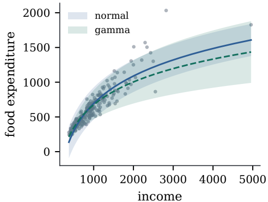
(b) two variance functions
