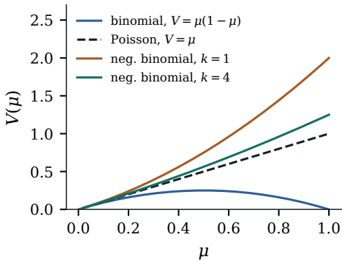
(b) bounded and overdispersed
