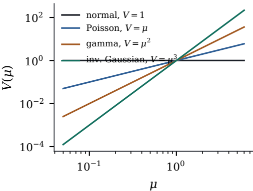
(a) the power family
