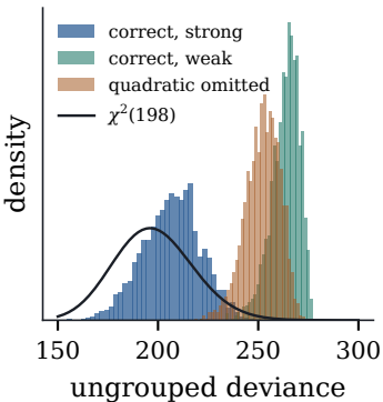
(a) null distribution
