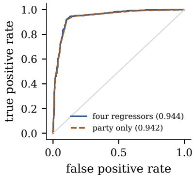
(c) ROC curves
