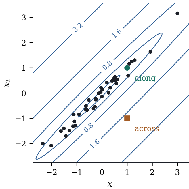
Figure 19.6.1: Standard deviation of the fitted mean, in units of \sigma , over the regressor plane for Example (Predicting along and across the pattern), with the 40 design points. The contours are elongated along the data: prediction at the circle, which follows the pattern, is precise; prediction at the square, which breaks it, is not.
