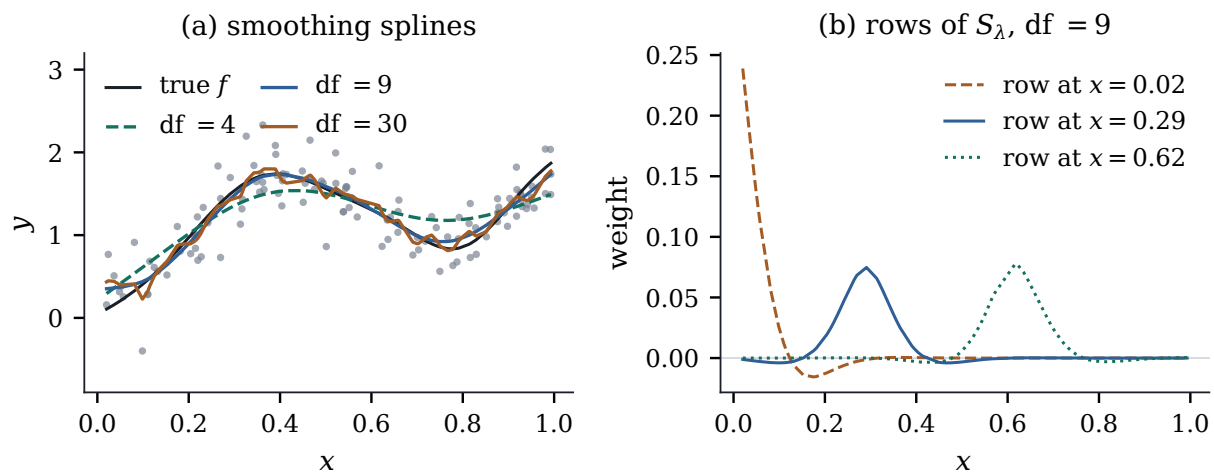
Figure 43.4.1: (a) Smoothing splines at three values of \lambda , labelled by effective degrees of freedom. (b) Three rows of S_\lambda at df = 9 , the weights producing \hat{f}(x) at x = 0.02 , 0.29 and 0.62 : local, summing to one, slightly negative beside the peak.
