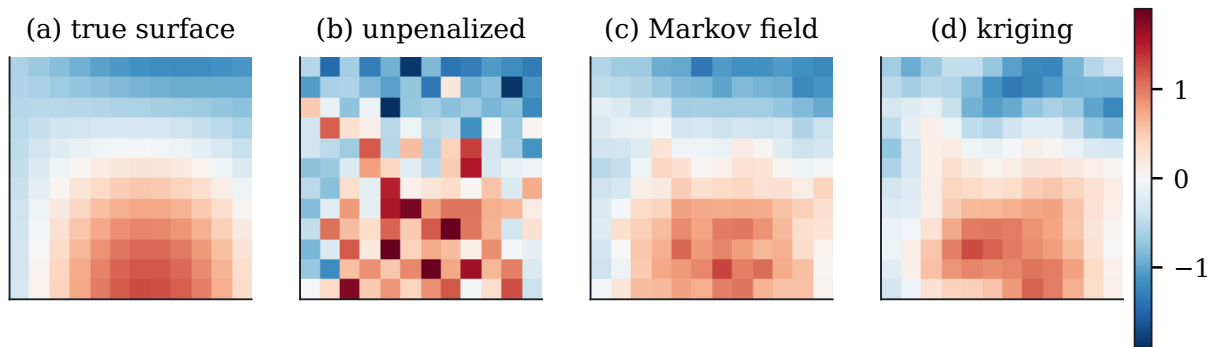
Figure 44.4.1: A simulated district map, all panels on one colour scale. (a) the surface used to generate the data. (b) unpenalized district effects. (c) the Markov random field Eq. 44.4.2 . (d) a kriging term on 21 knots.
