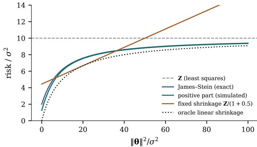
Figure 27.5.1: Risk of estimators of ten normal means with \sigma = 1 , against \|\boldsymbol{\theta}\|^2 : the unbiased estimator \mathbf{Z} , James–Stein (exact, from the Poisson mixture), its positive part (simulated, 4000 draws per point), a fixed proportional shrinkage, and the best linear shrinkage for each \boldsymbol{\theta} .
