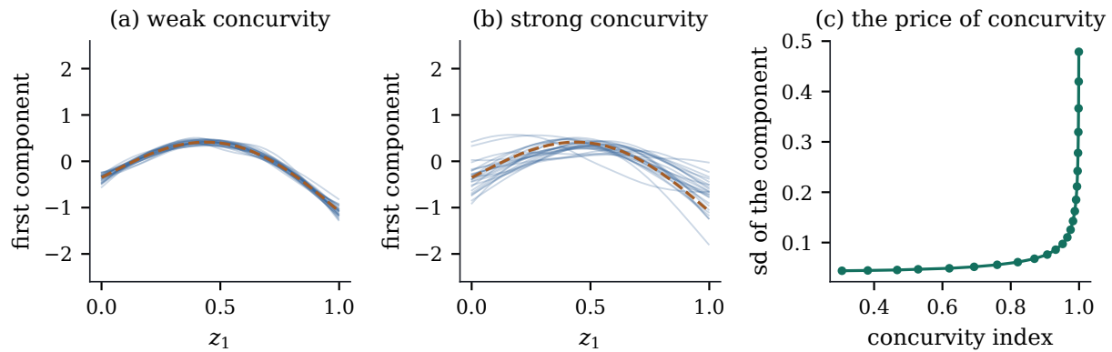
Figure 44.2.2: Concurvity. (a) and (b) twenty-five replicate estimates of the first component (truth dashed) under weak and strong dependence. (c) its exact standard deviation at z_1 = 0.3 against the concurvity index Eq. 44.2.5 .
