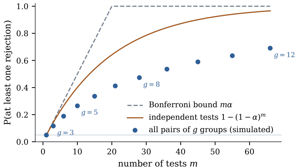
Figure 13.1.1: Probability of at least one false rejection among m unadjusted level-0.05 tests: all pairs of g = 2, \dots, 12 equal means (dots, simulated), independent tests (curve, Eq. 13.1.1 ) and the Bonferroni bound m\alpha (dashed).
