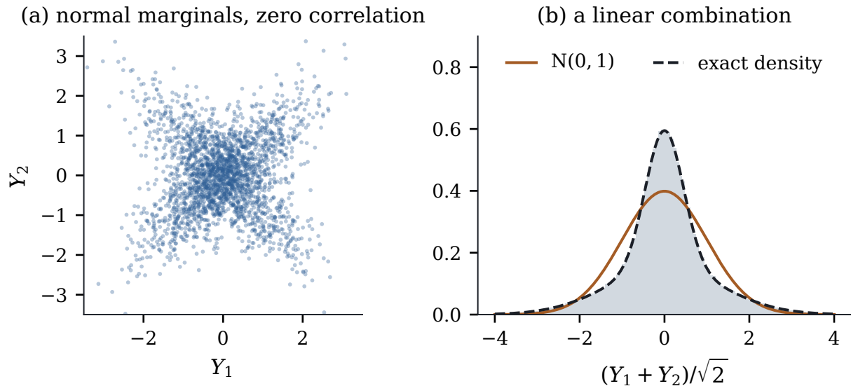
Figure 3.3.1: An equal mixture of bivariate normals with correlations \pm 0.8 . (a) Both margins are exactly N(0,1) and the correlation is zero, but the scatter is an X, not an ellipse. (b) The linear combination (Y_1 + Y_2)/\sqrt{2} has variance one but is sharply peaked and heavy-tailed compared with N(0,1) . By Definition 3.1.1, one non-normal direction is enough to rule out joint normality.
