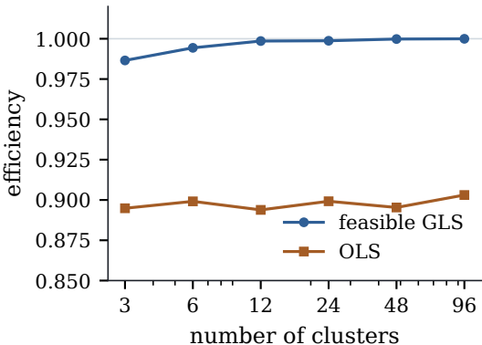
(a) efficiency relative to GLS
