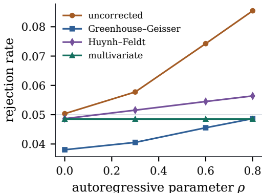
(b) level of a 5% test
