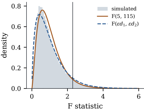
(a) null distribution, \varepsilon = 0.70
