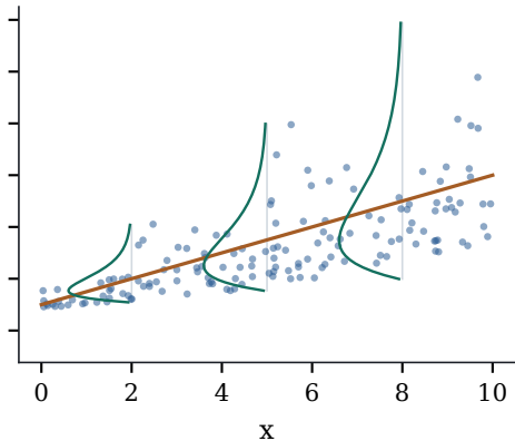
(b) same mean, other distribution
