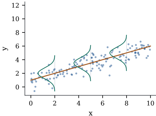
(a) linear model assumptions hold
