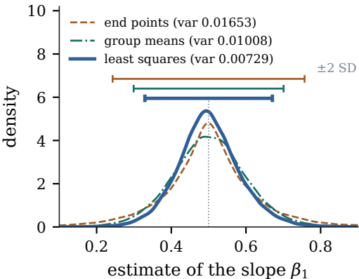
(a) three linear unbiased estimators
