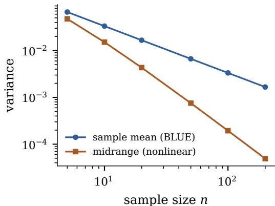
(b) uniform errors
