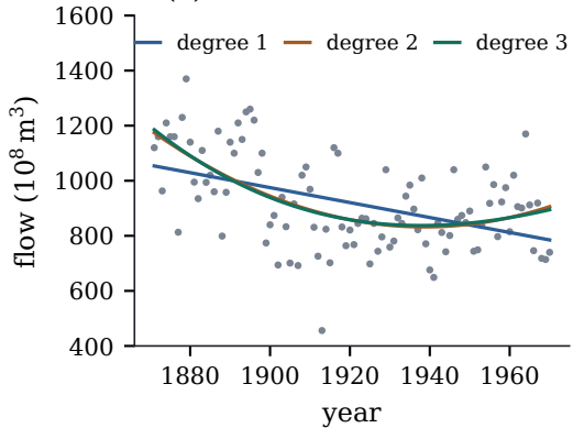
(b) Nile flow and nested fits
