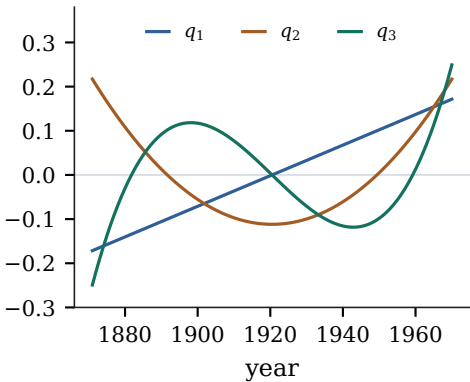
(a) orthonormal polynomials
