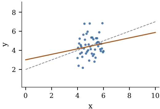
(a) narrow range: R^2 = 0.03
