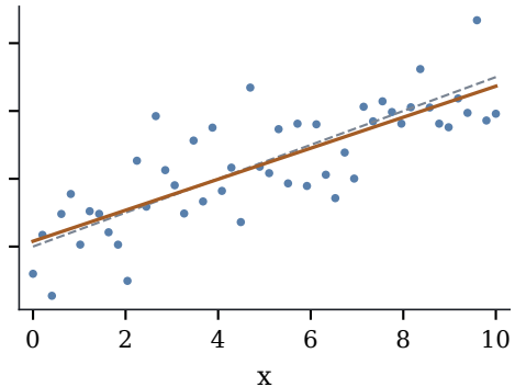
(b) wide range: R^2 = 0.63
