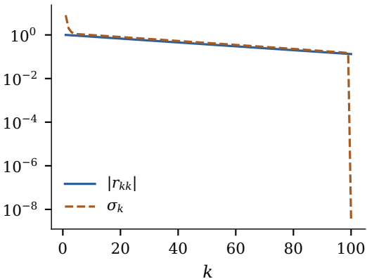
(a) Kahan's matrix
