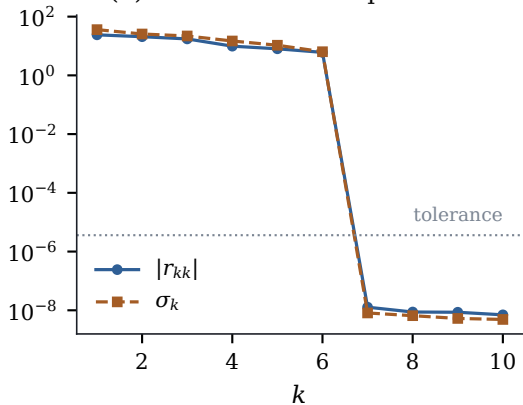
(b) numerical rank 6 plus noise
