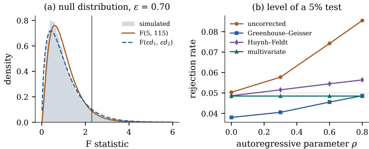
Figure 33.3.1: (a) The null distribution of the uncorrected F statistic with autoregressive errors, against the nominal F(5, 115) density and the moment-matched F(\varepsilon d_1, \varepsilon d_2) of Proposition 33.3.3, with the nominal 5% point marked. (b) Simulated level of four tests as \rho grows.
